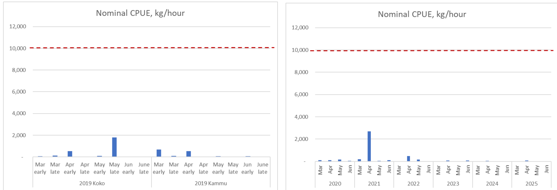
Fig. 1. Time series of the nominal CPUEs from the monitoring survey for North Pacific armorhead in the Koko and Kammu Seamounts in 2019-2025. The red dash line indicates the threshold level of 10 t/hour which is one of the criteria for high recruitment.
